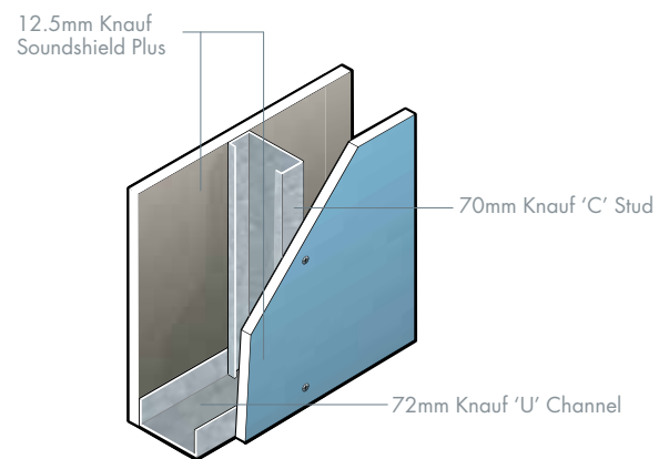
Knauf Soundshield Plus solution for Approved Document E – Internal wall 40dB(Rw)
